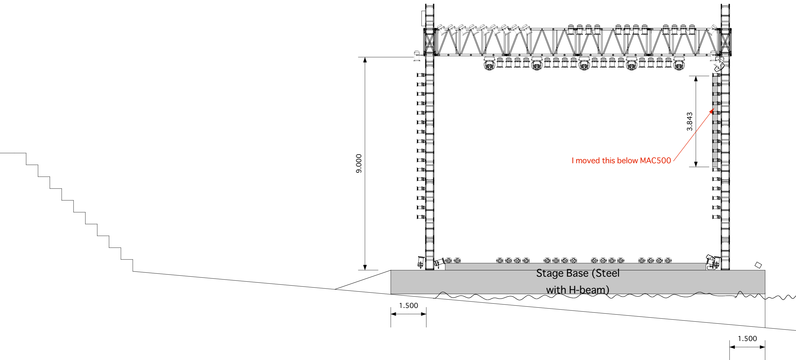
GOSUNG Seaside 2004 Lighting Plot <Side view of Lighting equipments> <1/80>
